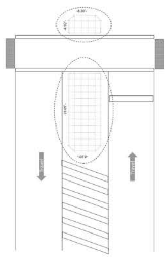
Full Pedestrian Refuge Median @ Intersection
