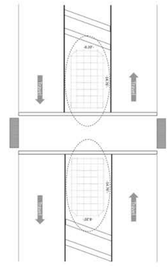
Full Pedestrian Refuge Median @ Mid-Block
