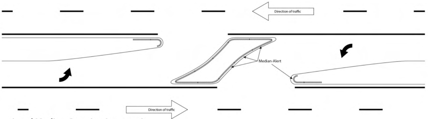
Directional Median Opening Intersection
